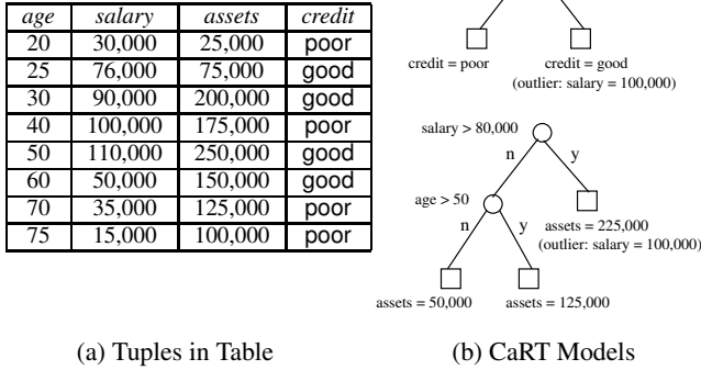
Figure 1: Model-Based Semantic Compression.
